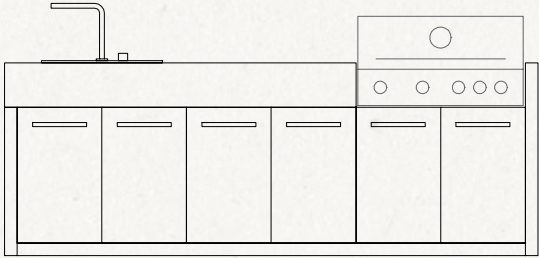
three 252 X 70 X 91 cm
